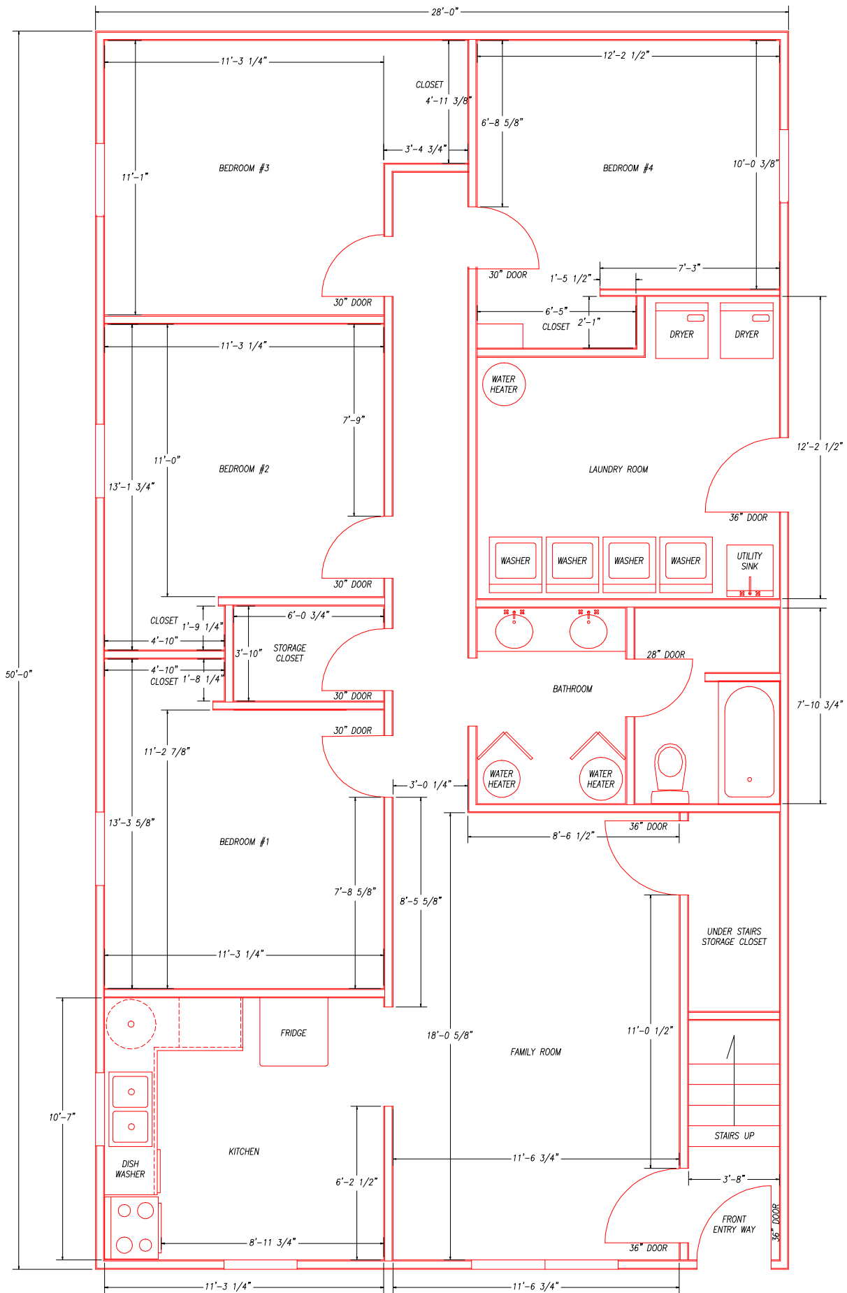
APARTMENT A
